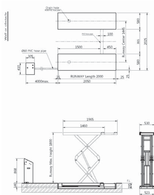
IN-GROUND INSTALL
