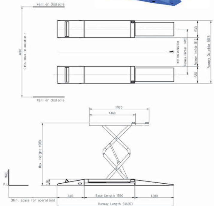
ON-GROUND INSTALL
