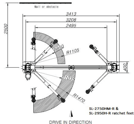
RATCHET ARM
