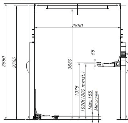
SL-2750HM & SL-2950H STANDARD FOOT
