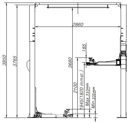
SL-2750HM-R & SL-2950HR RATCHET FOOT
