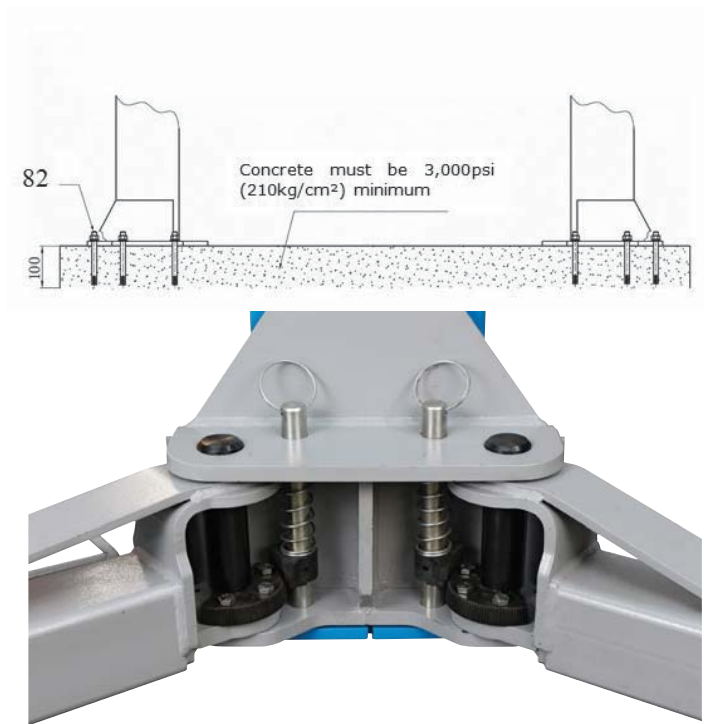
AUTOMATIC LOCKING PINS
