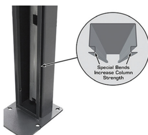
UNIQUE 'S' BEND POST DESIGN
