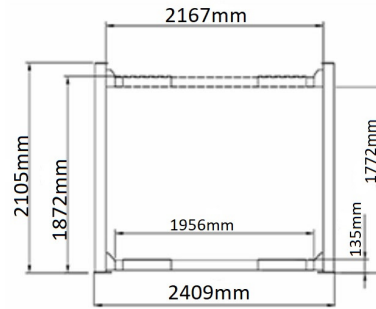
3000kg Compact 4 Post Parking Lift
