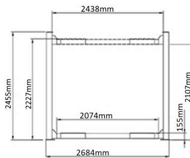
3500kg 4 Post Parking Lift
