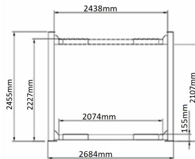
3500kg High lift 4 Post Parking Lift
