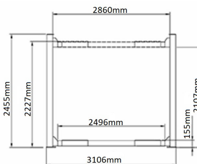
4000kg Large 4 Post Parking Lift
