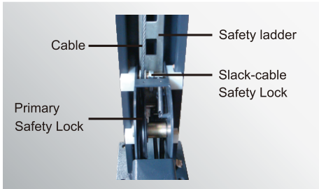
Double safety locks provide additional safety.
